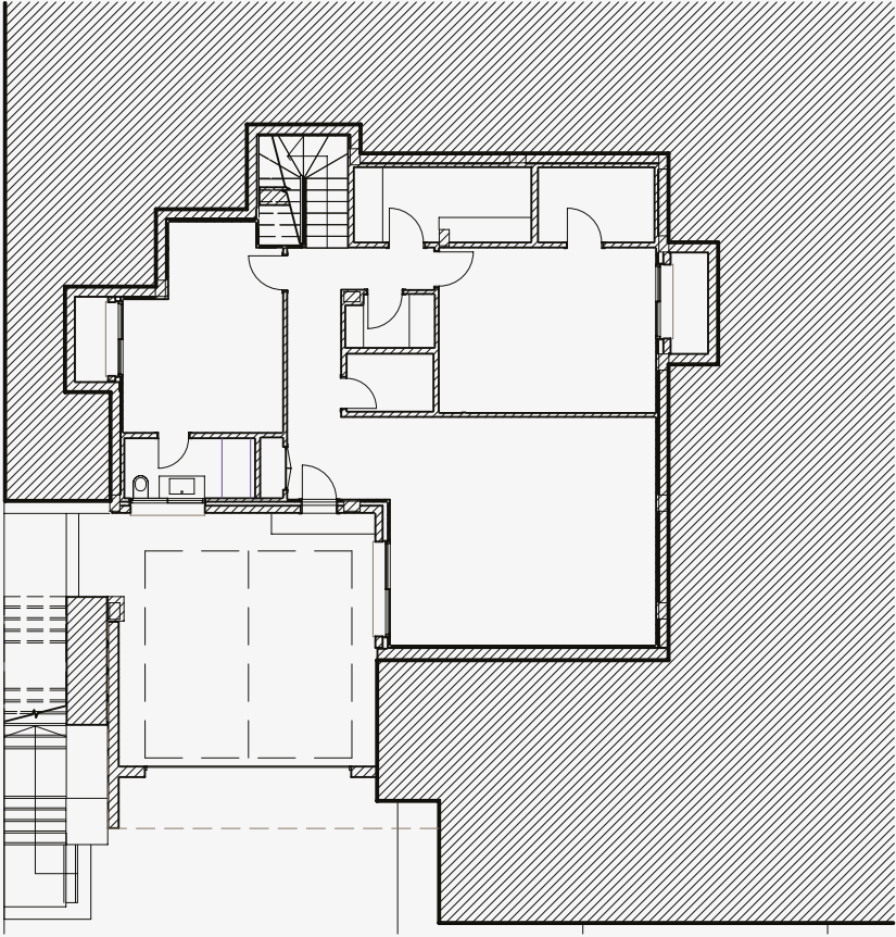
BASEMENT FLOOR
