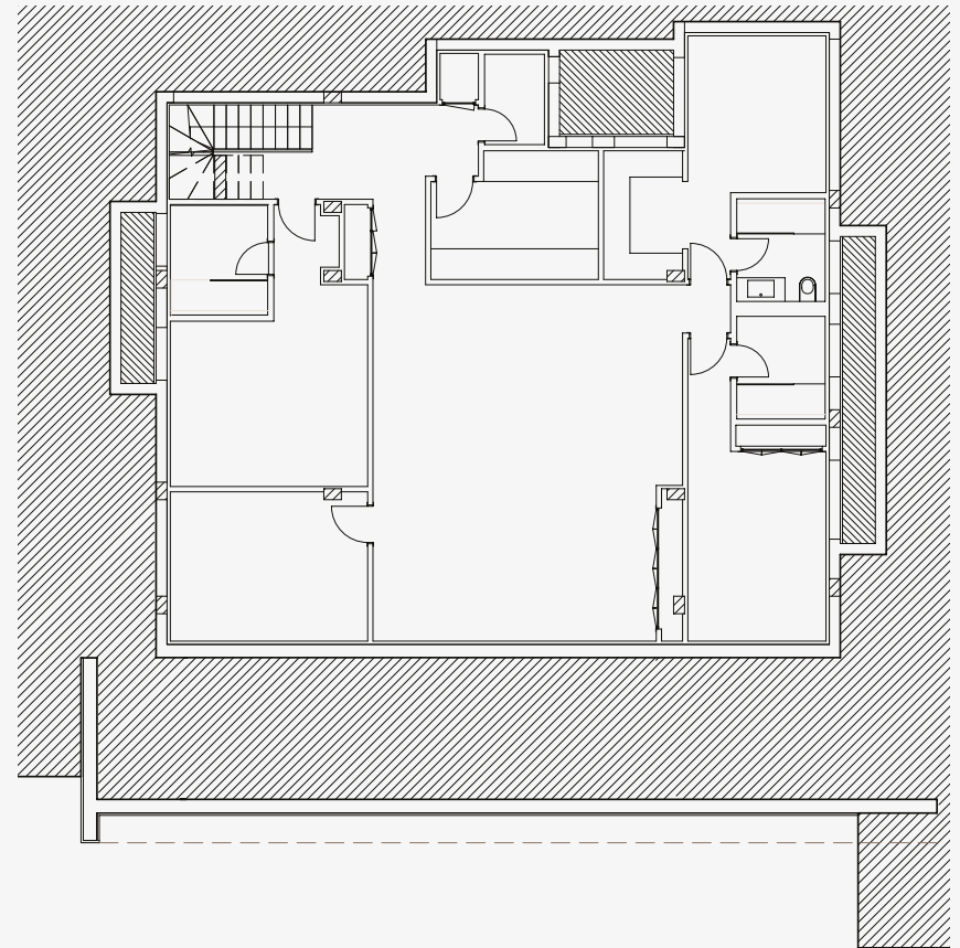
BASEMENT FLOOR
